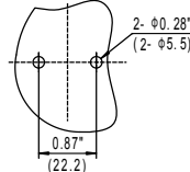
Rear Bracket Mount
