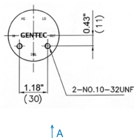
Rear Bracket Mount
